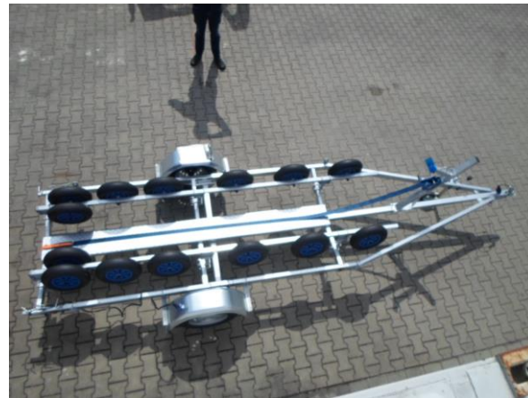
Rollenbahn-Trailer
